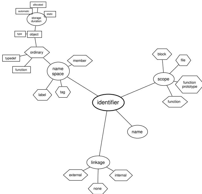
Figure .1: Attributes a C language identifier can have.
